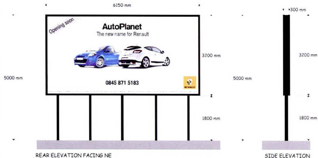
REAR ELEVATION FACING NE
