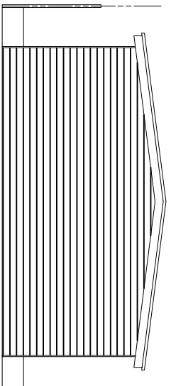
NORTH ELEVATION
