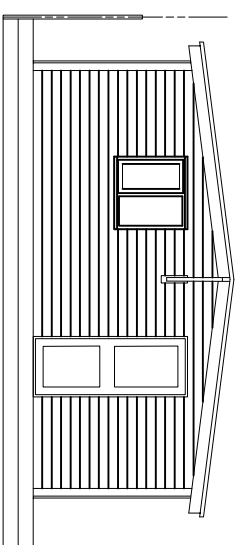
SOUTH ELEVATION
