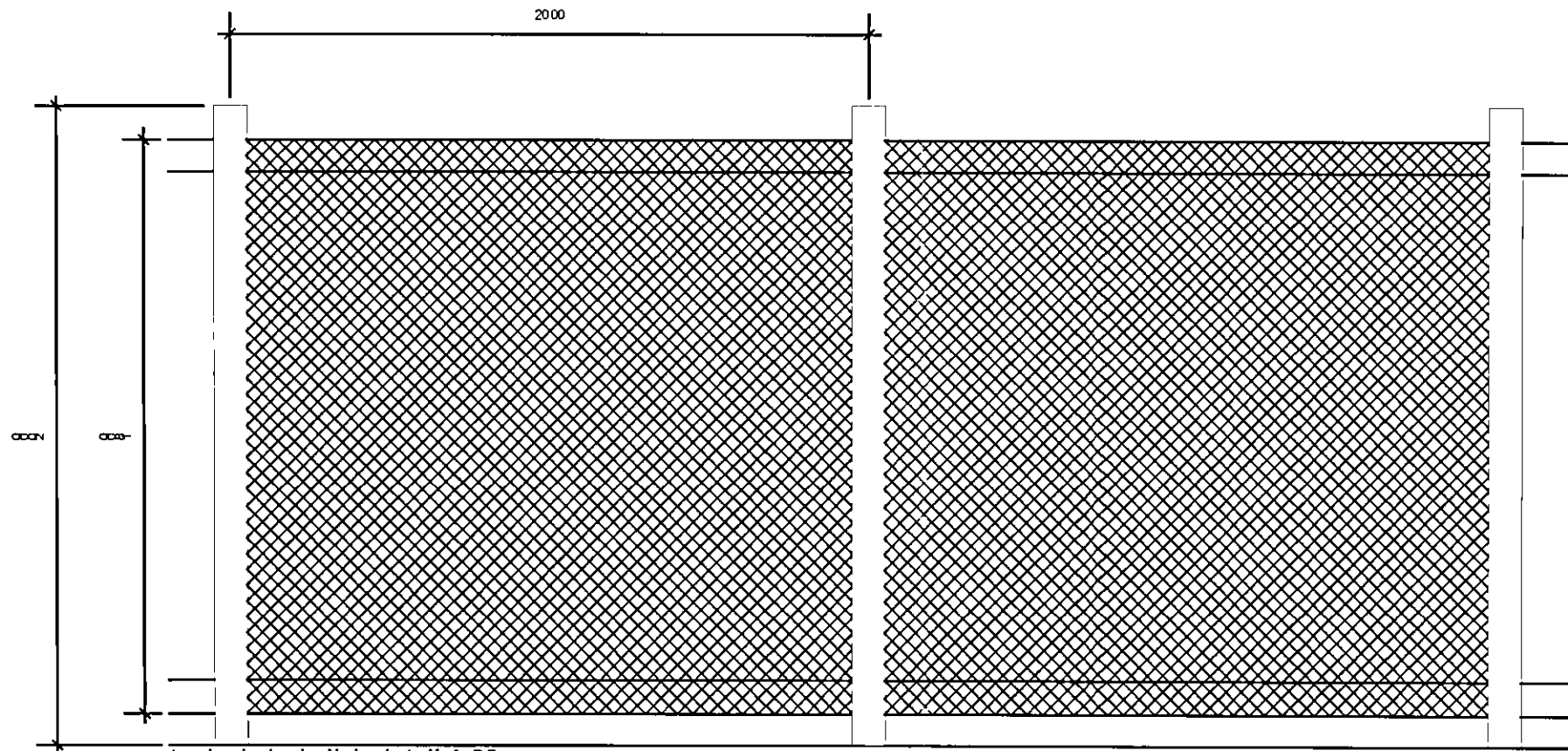
typical chain link detail 1:20
