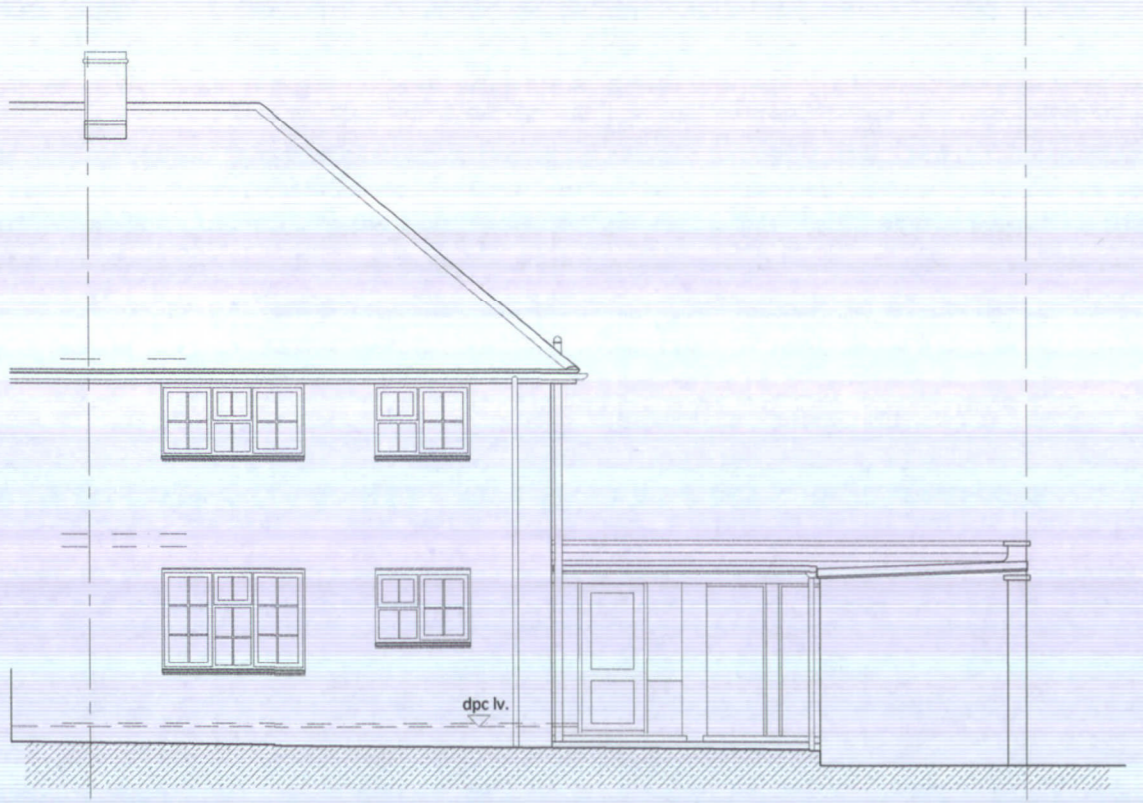
REAR ELEVATION FACING N-E AS EXISTING
