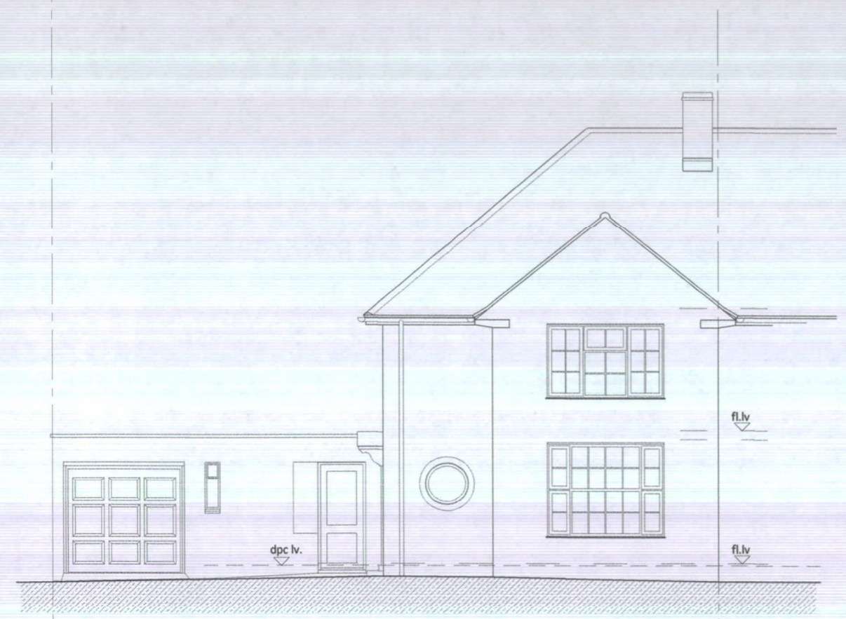
FRONT ELEVATION FACING S-W AS EXISTING
