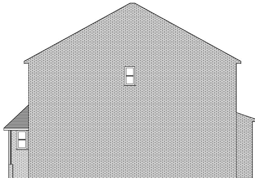
NORTH SIDE ELEVATION AS EXISTING
