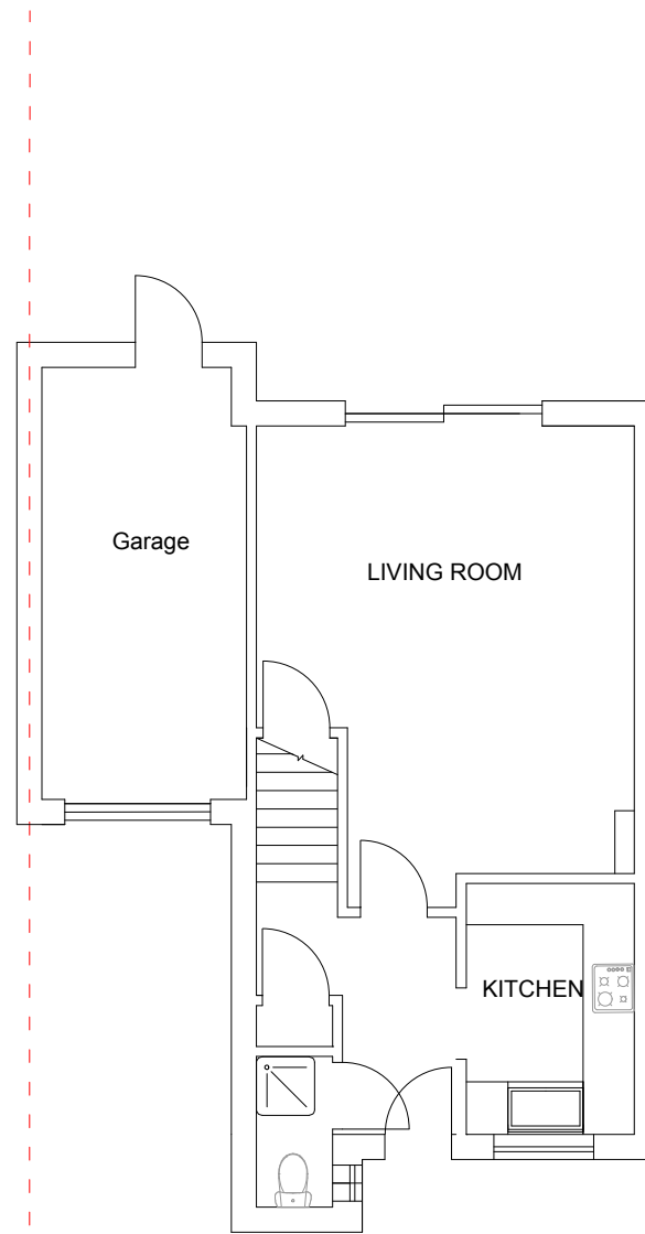
GROUND FLOOR PLAN AS EXISTING
