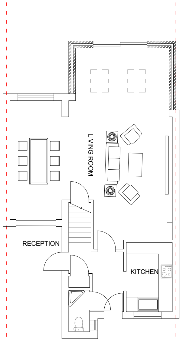
GROUND FLOOR PLAN AS PROPOSED
