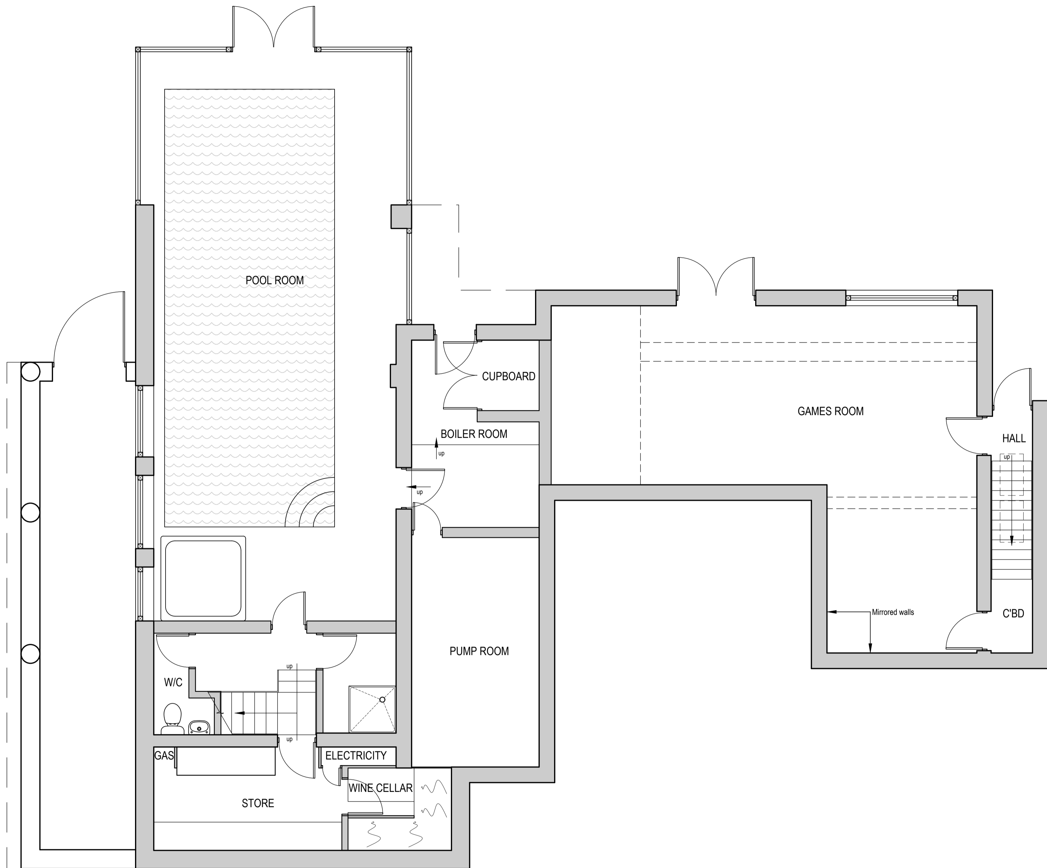
EXISTING LOWER GROUND FLOOR PLAN (scale 1:50)
