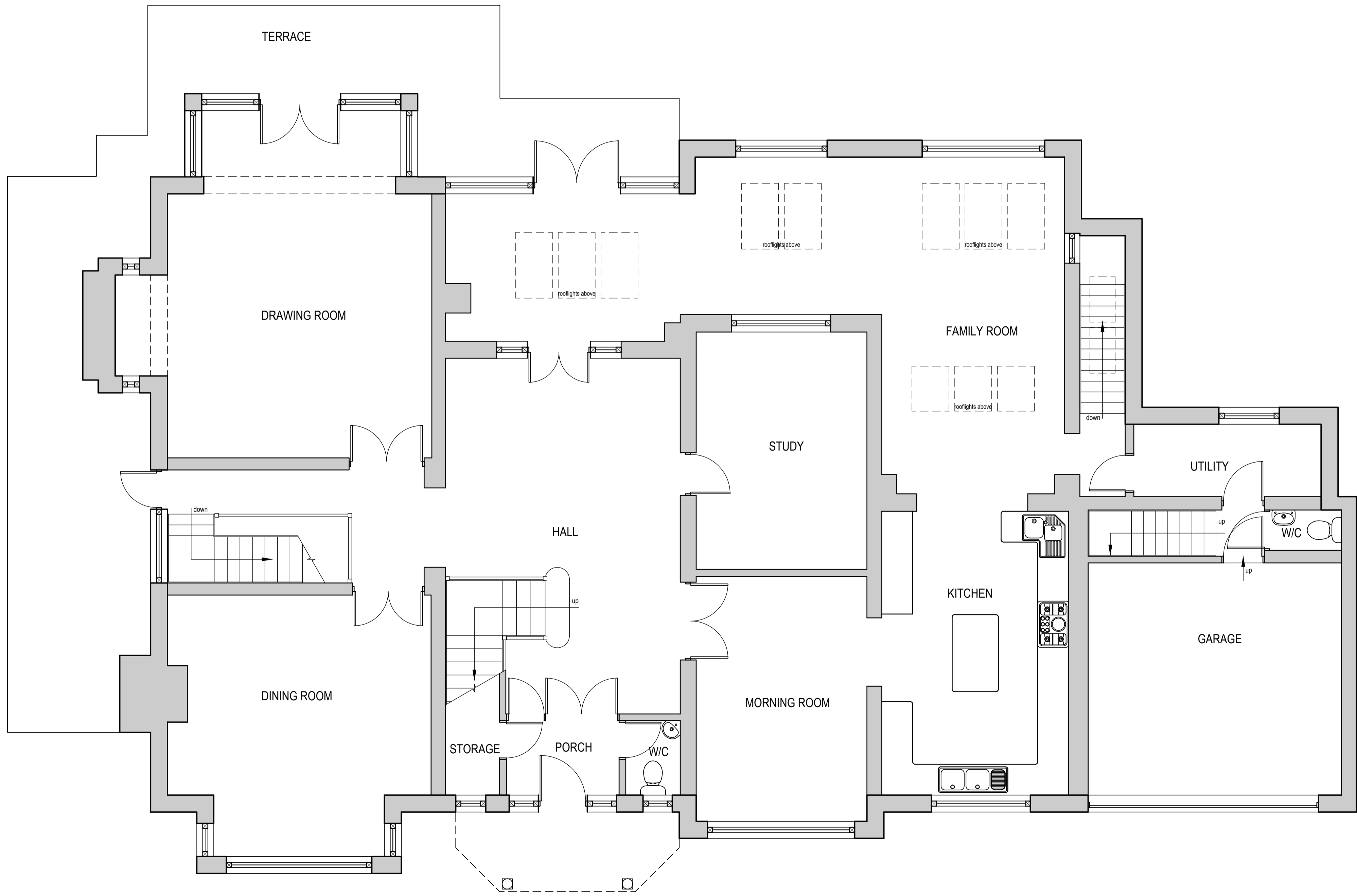
EXISTING GROUND FLOOR PLAN (scale 1:50)
