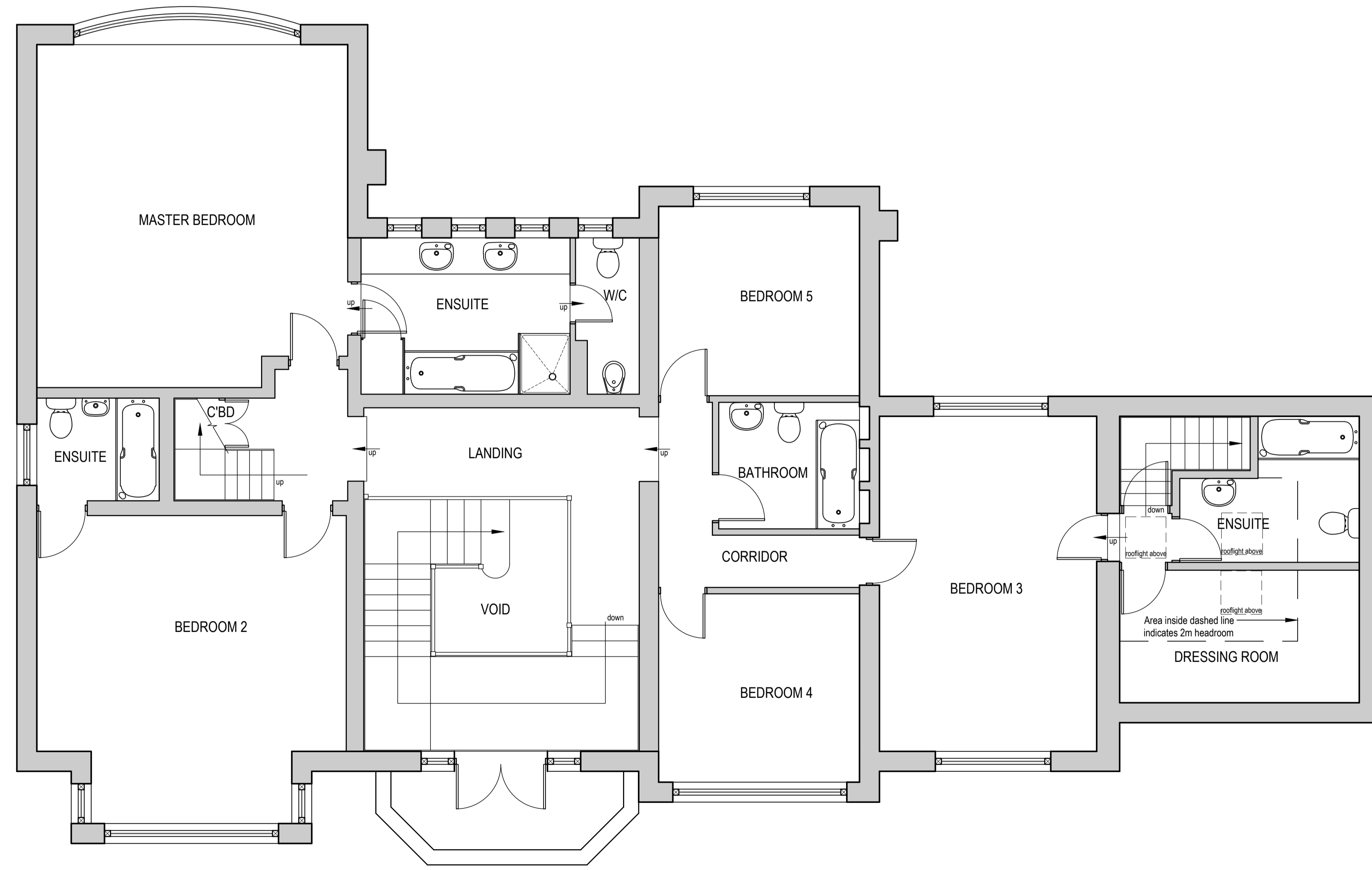
EXISTING FIRST FLOOR PLAN (scale 1:50)
