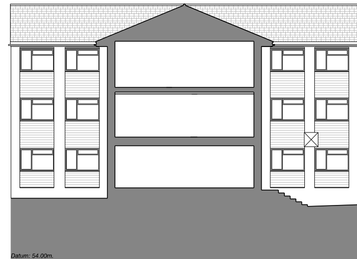
03 Existing Elevation 6 1:200@A3
