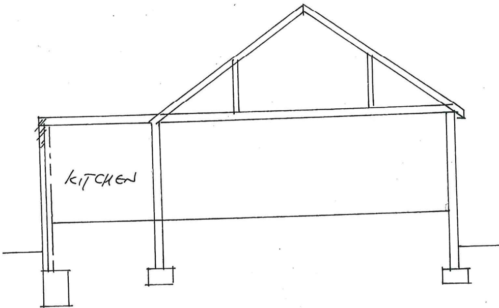
PROPOSED SECTION
