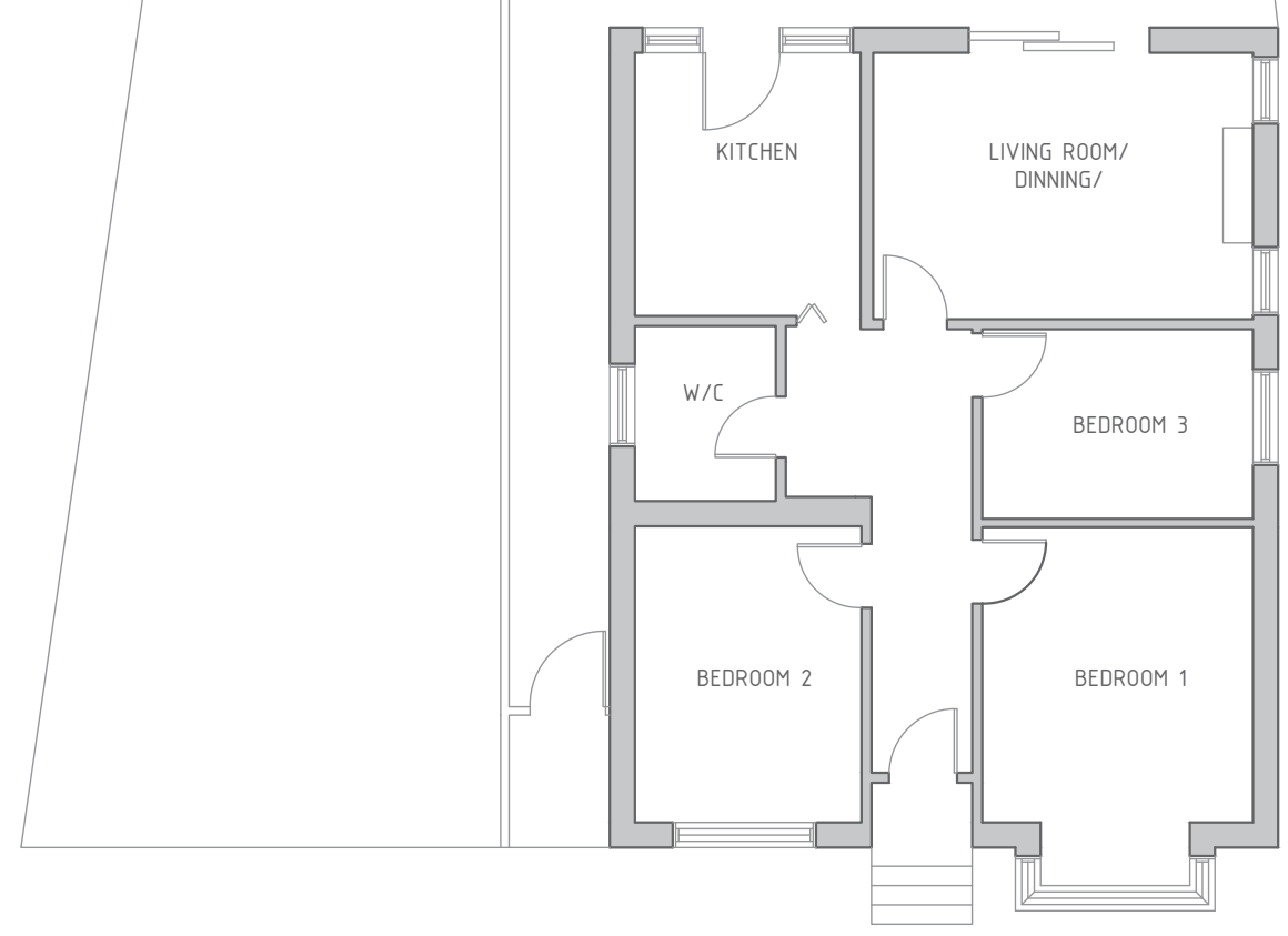
FLOOR PLANS
