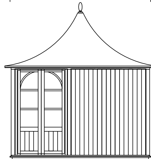
Side Elevation (West)
