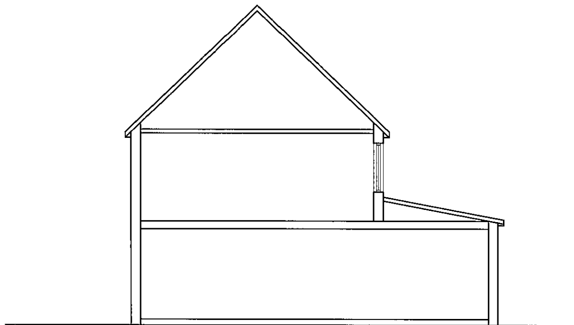
EXISTING SECTION
