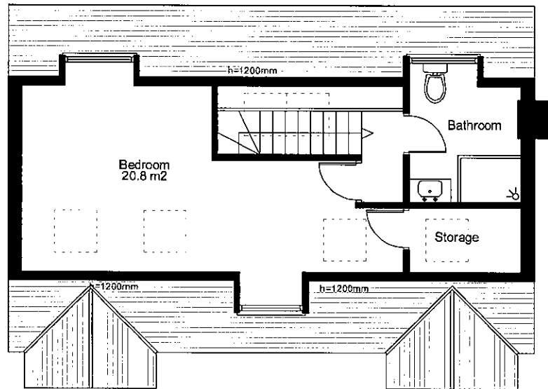
PROPOSED LOFT FLOOR
