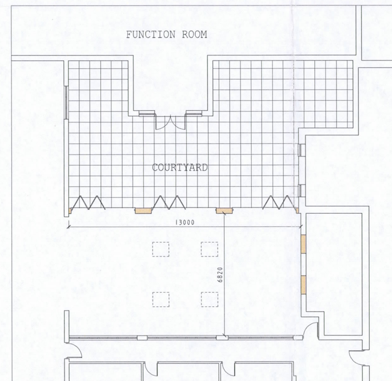
PROPOSED COURTYARD PLAN
