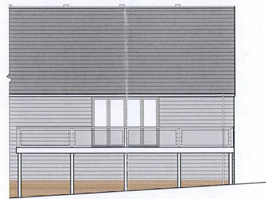
PROPOSED ELEVATION TERRACE A
