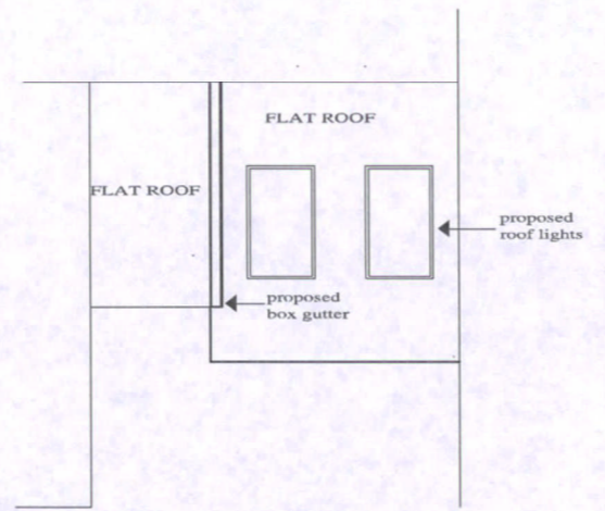
PROPOSED PART ROOF PLAN
