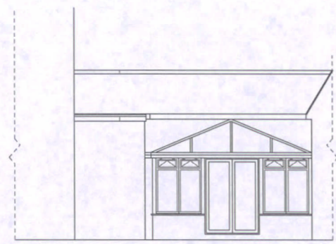
EXISTING PART ELEVATION
