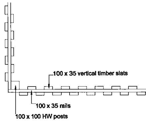
New Fence Plan
