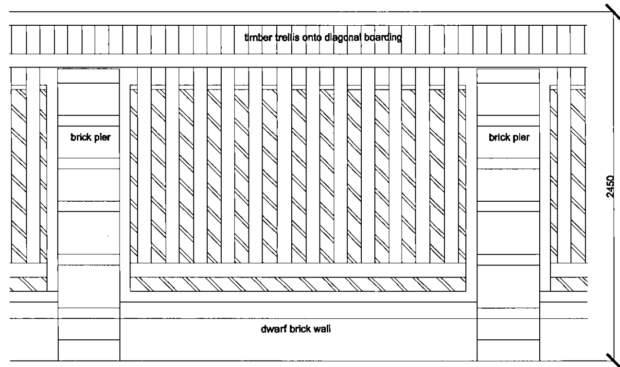
Existing Elevation B
