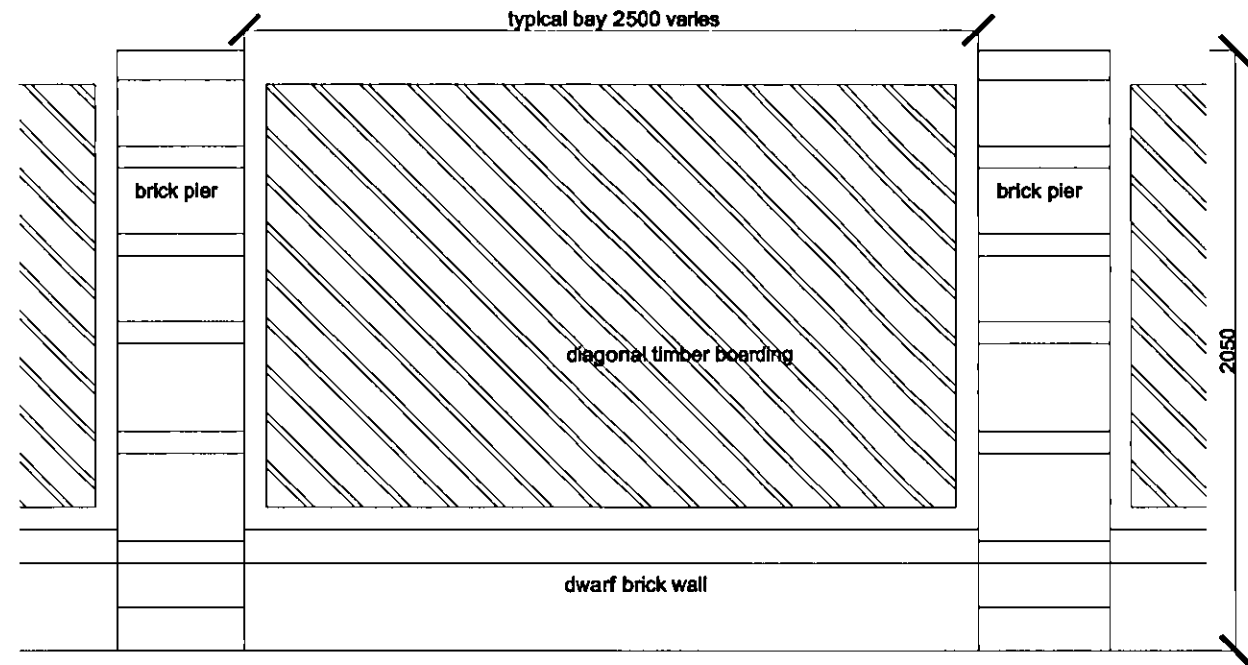
Existing Elevation A
