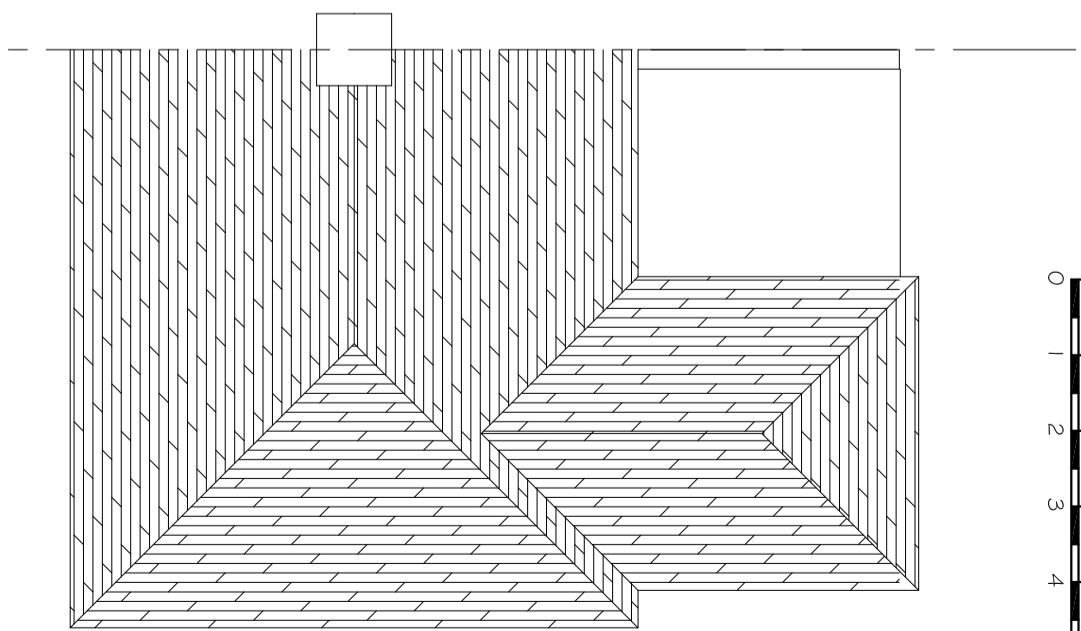
ROOF PLAN
