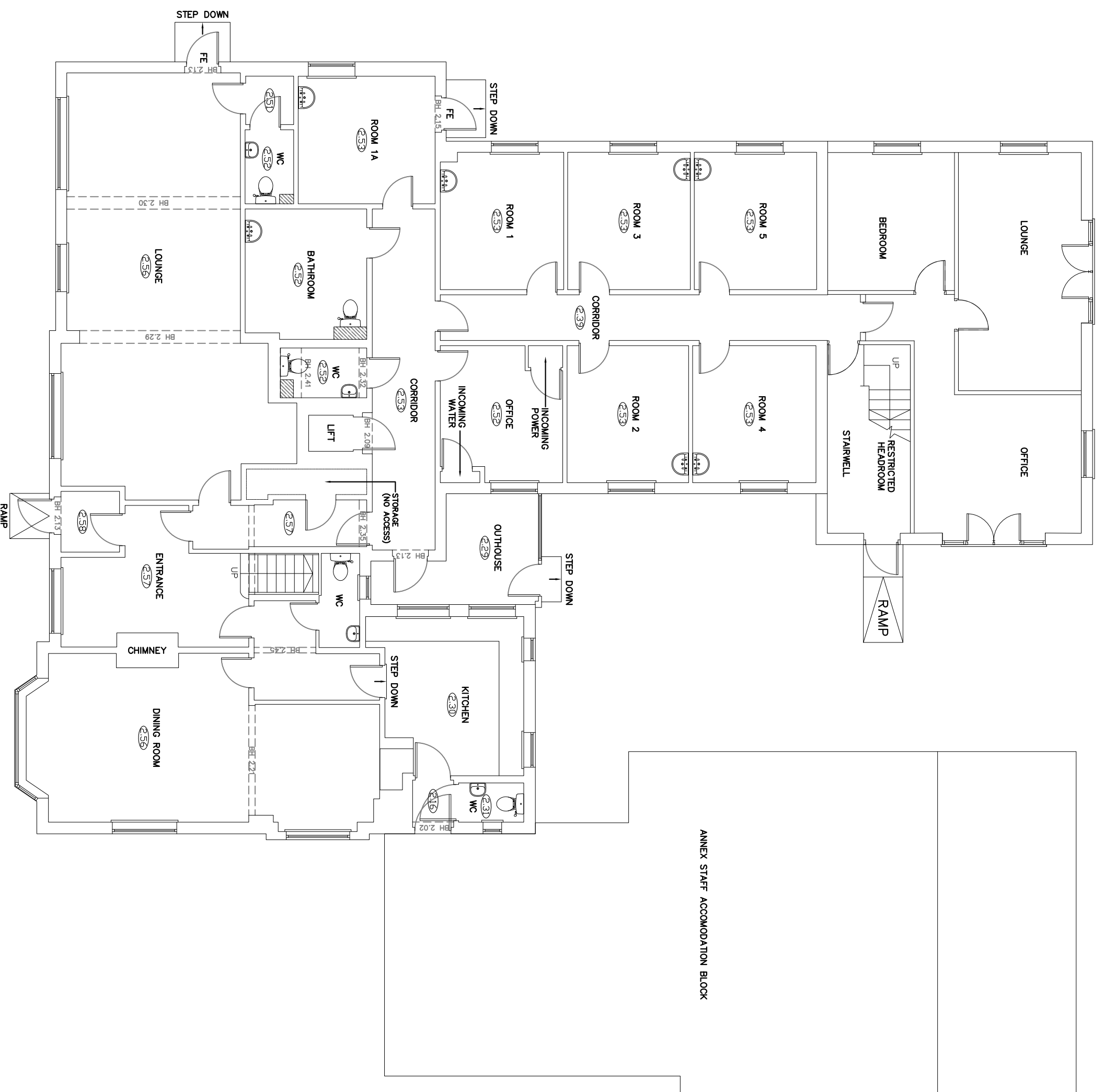
GROUND FLOOR
