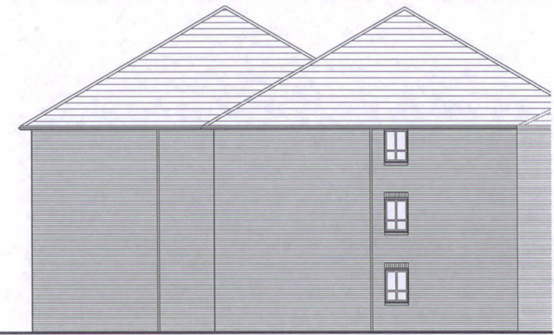
NORTH ELEVATION
