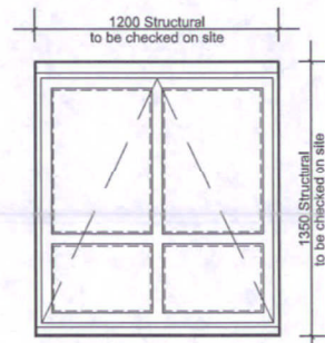
PROPOSED UPVC WINDOWS
