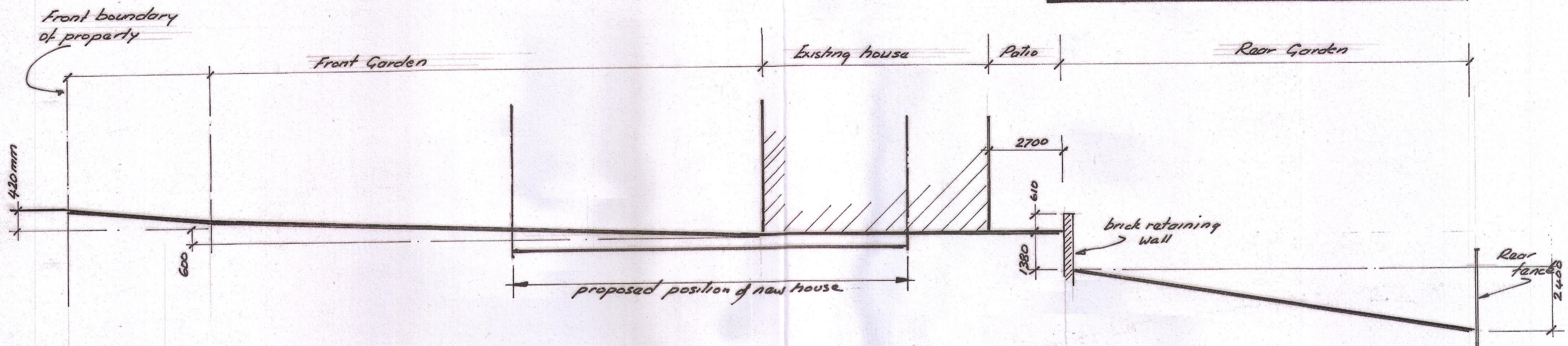
Section thro' Existing site with existing house Position 1:100 and Proposed Position of New house
