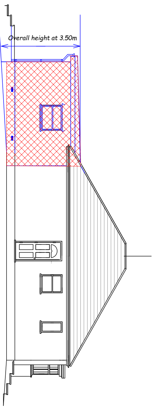
Proposed side elevation looking from No 19.
