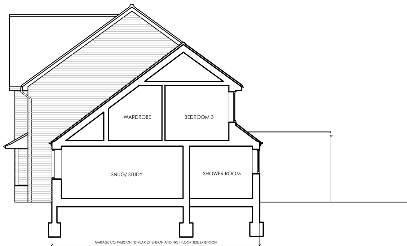
SIDE ELEVATION/ SECTION 1:100
