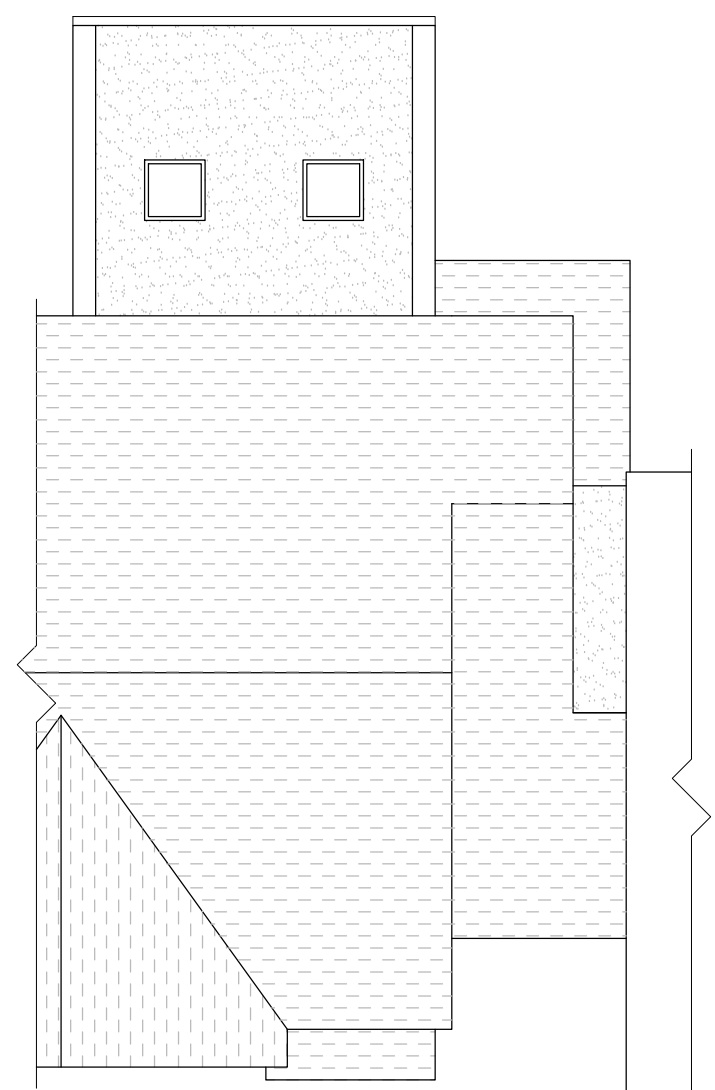
ROOF PLAN 1:100
