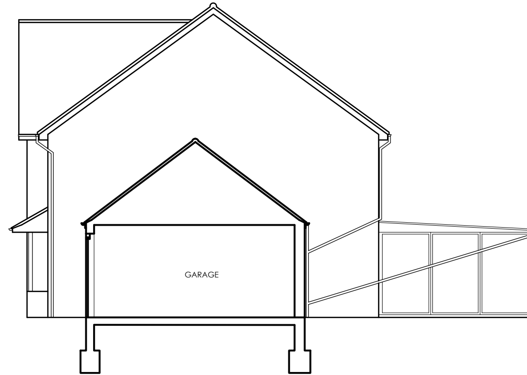
SIDE ELEVATION/ SECTION 1:100
