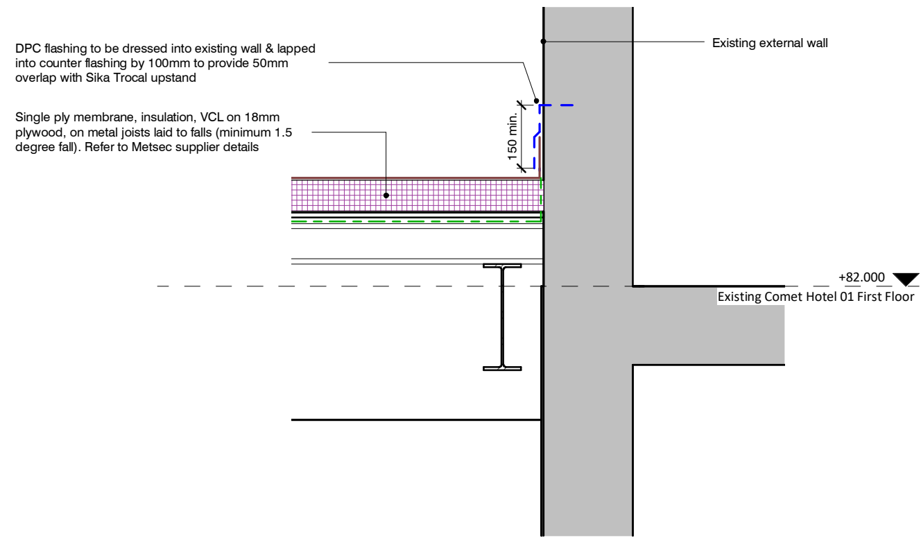
Existing parapet detail (solid wall construction) 1 : 20
