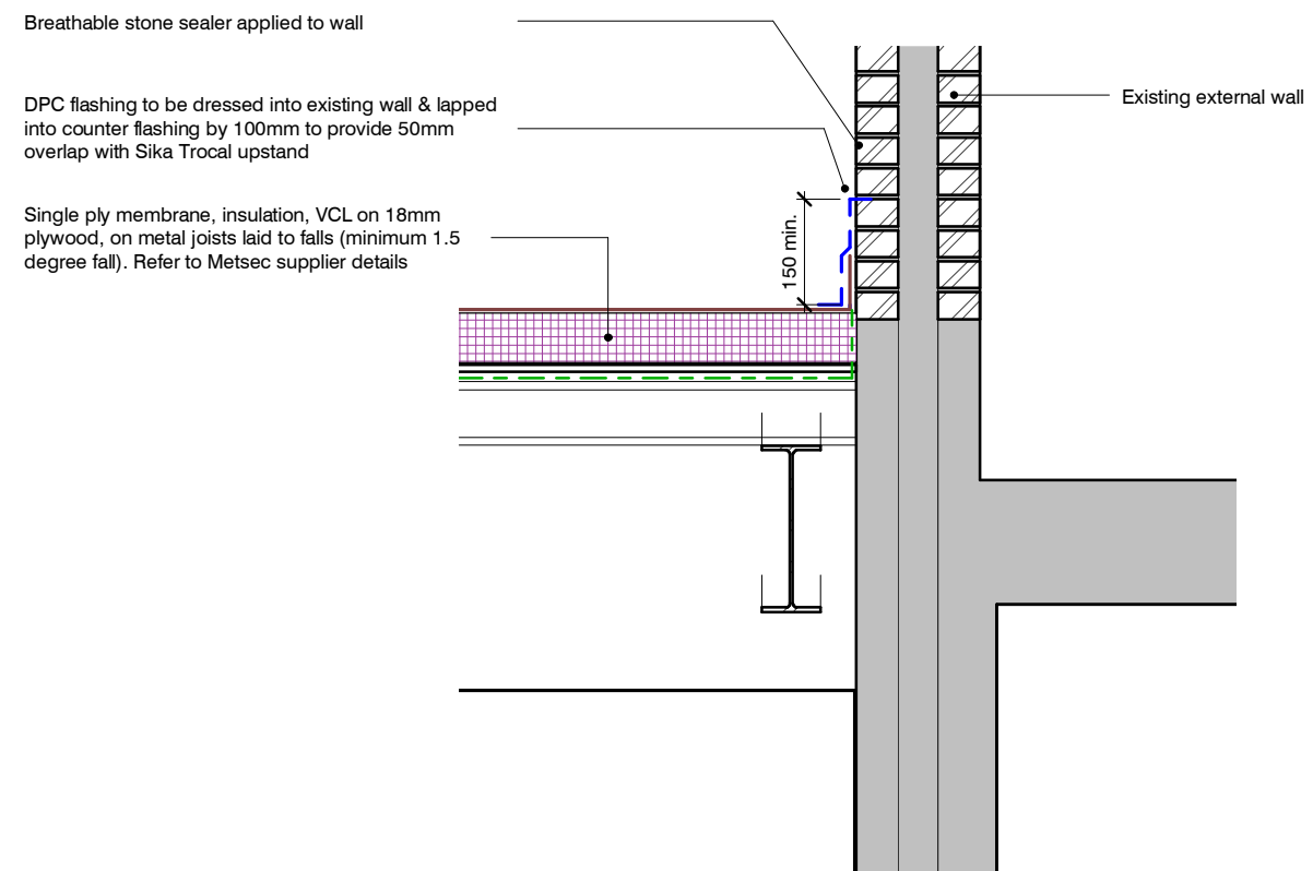
Existing parapet detail (cavity wall construction) 1 : 20
