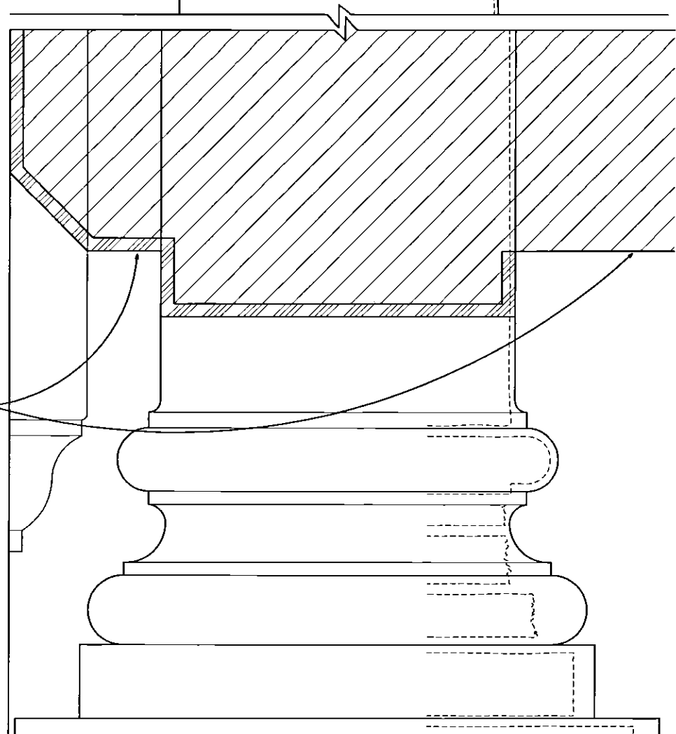
Capital, Entablature (A) & Base Mouldings
