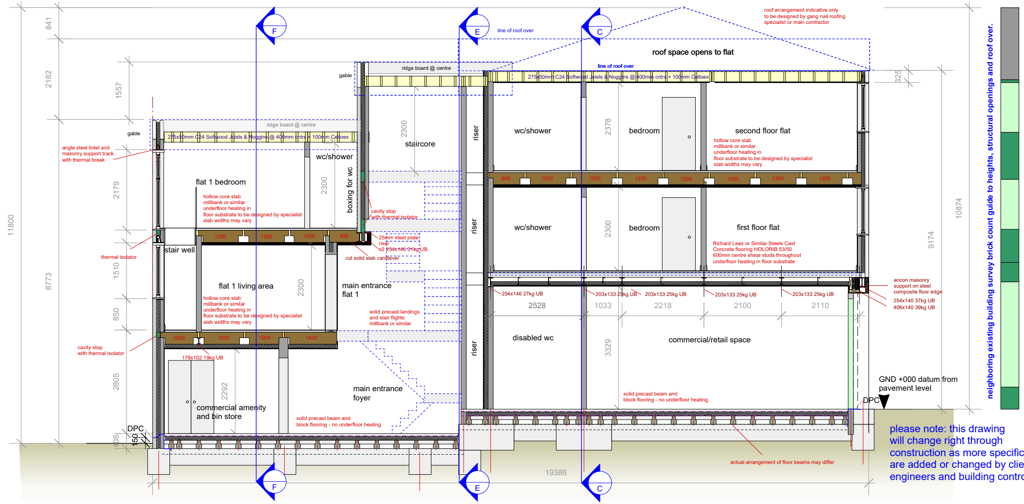
section G | through main building - north facing - detailing main stair core and service risers
