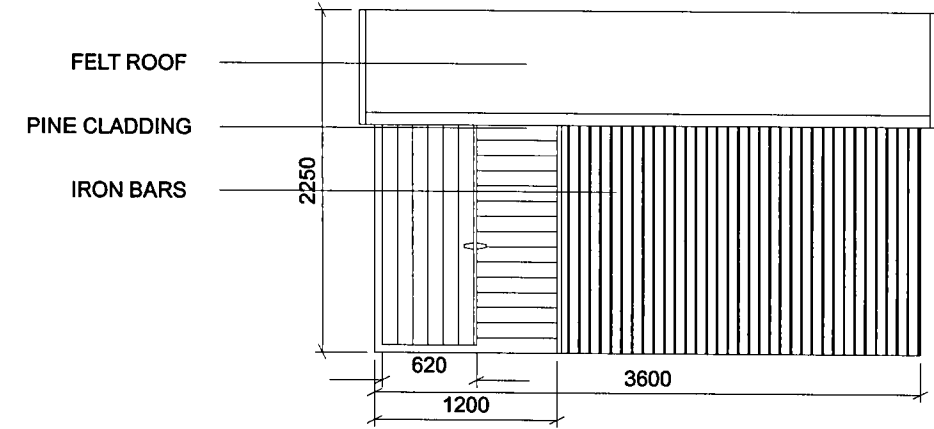
EAST ELEVATION
