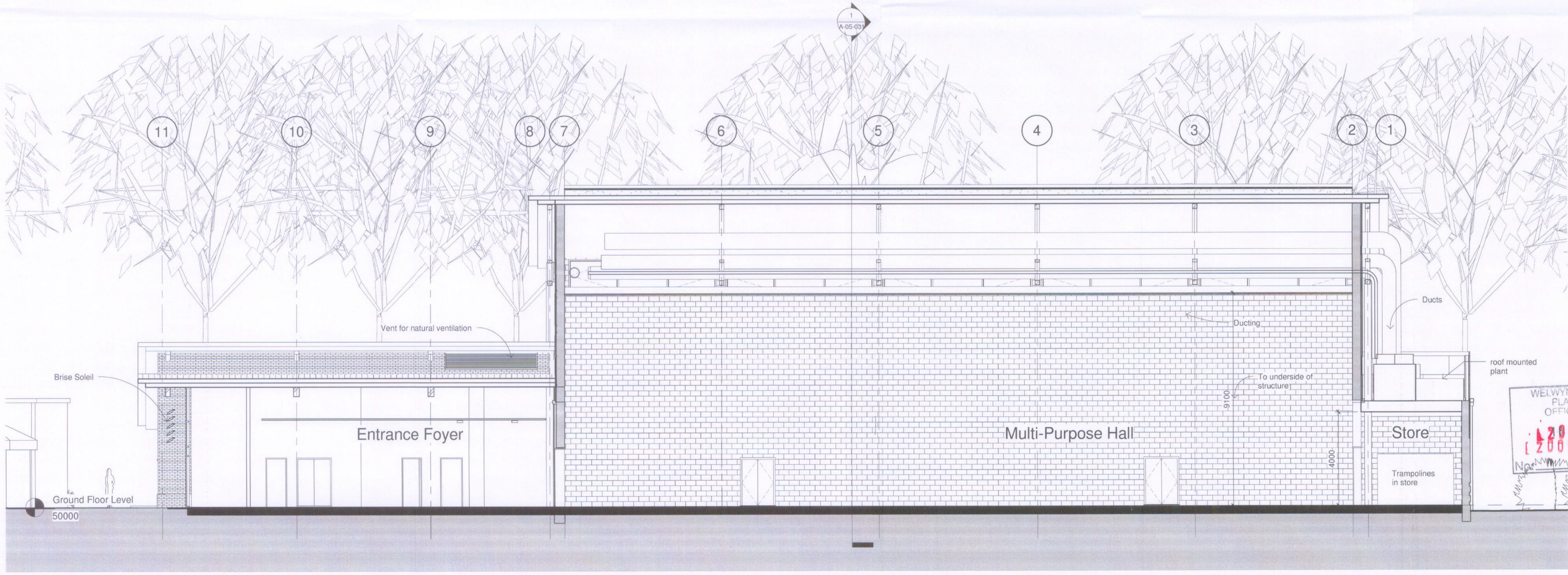
2 Section through whole building 1 : 100
