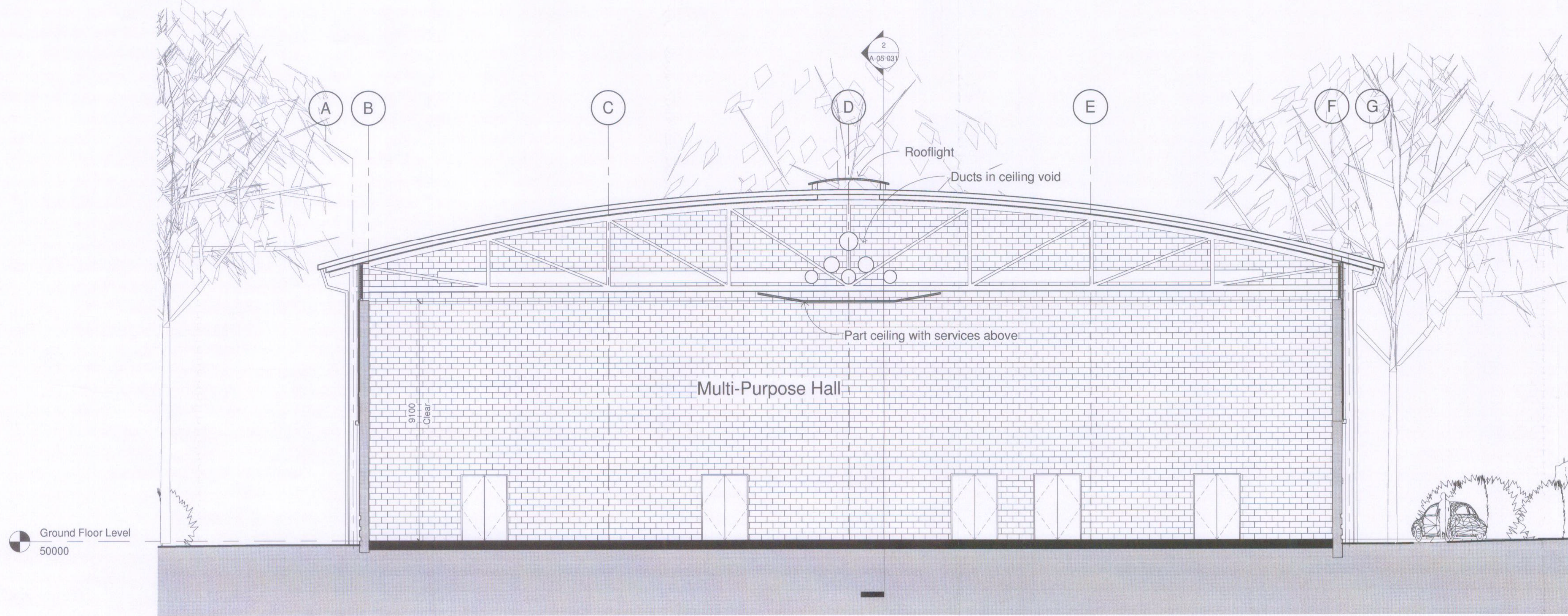
1 Section Through Sports Hall 1 : 100
