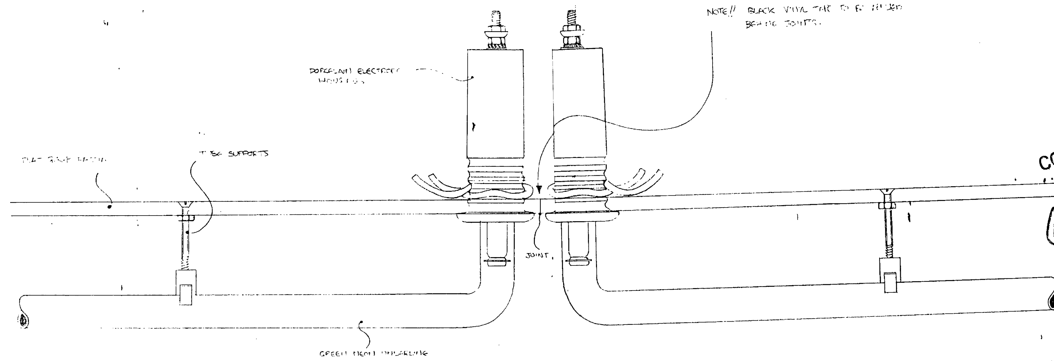
TYPICAL JOINT DETAIL FOR MARKS & SPECIFIER - WELWYN GARDEN CITY.
