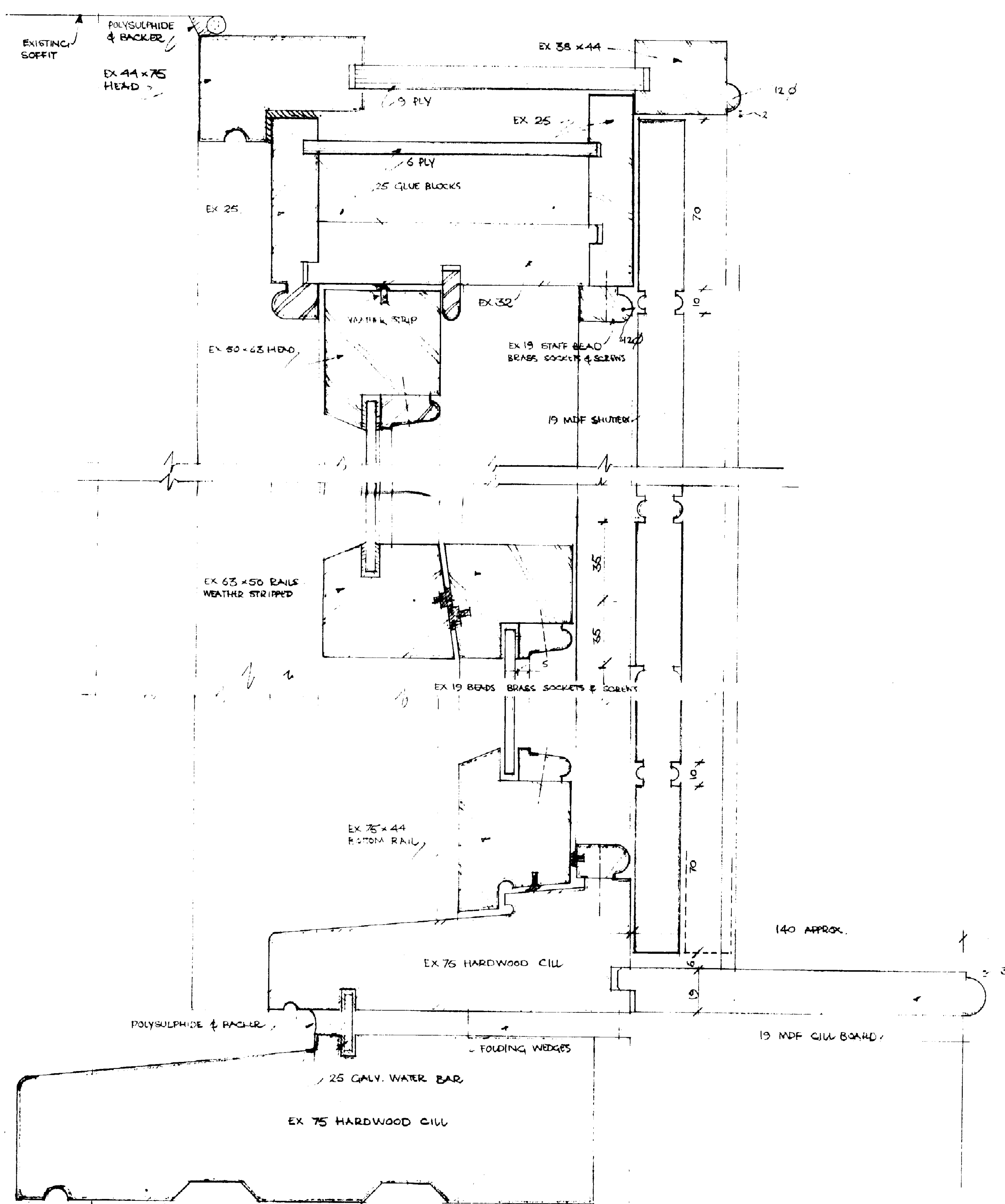
SECTION AA
