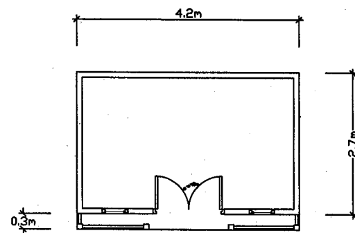
Floor Plan
