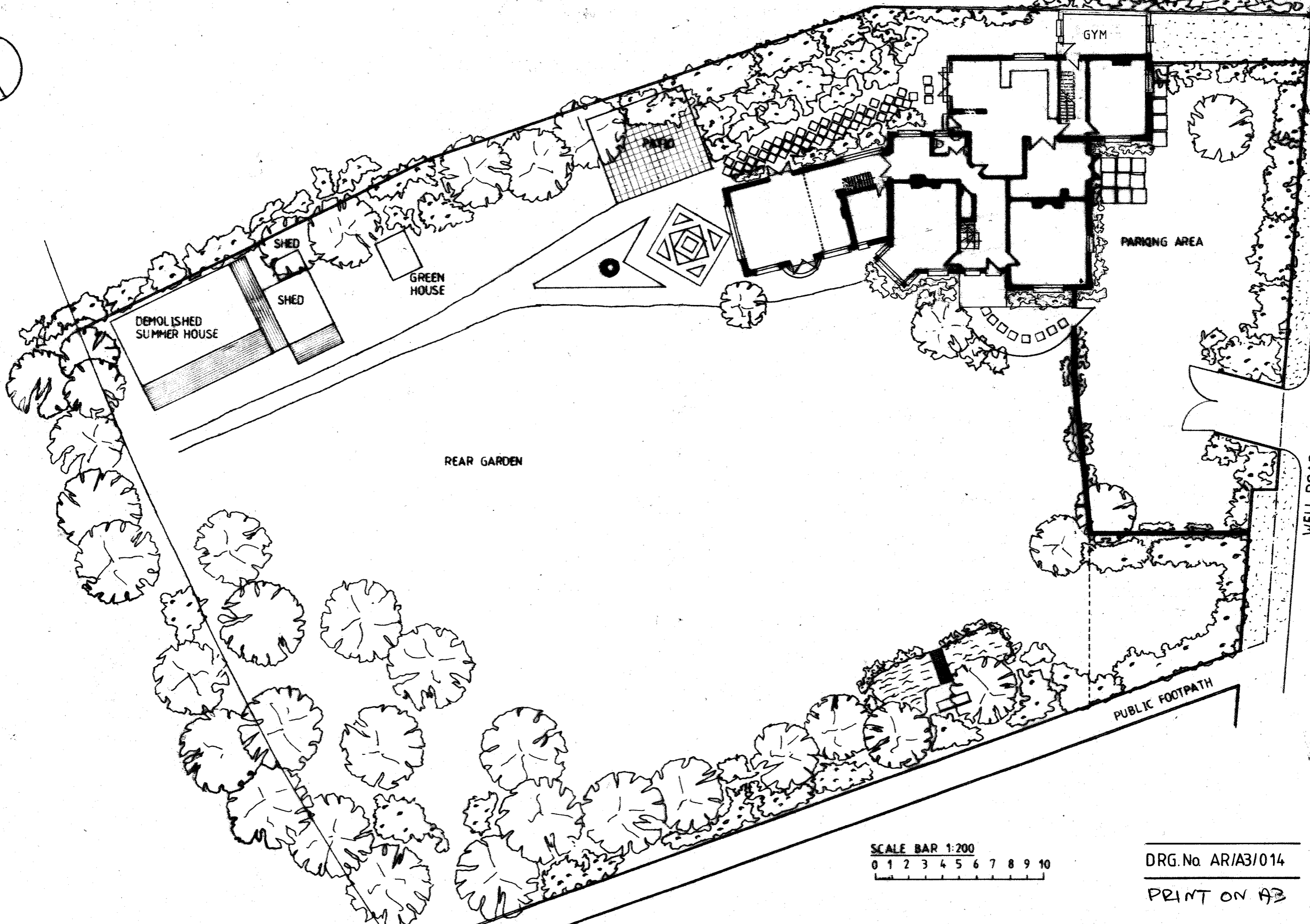
JUST HOUSE, COOPERS LANE EN6 4NJ - PROPOSED SITE PLAN - SCALE 1:200
