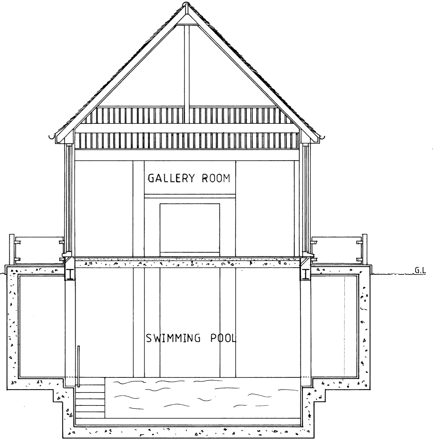
SECTION Z-Z
