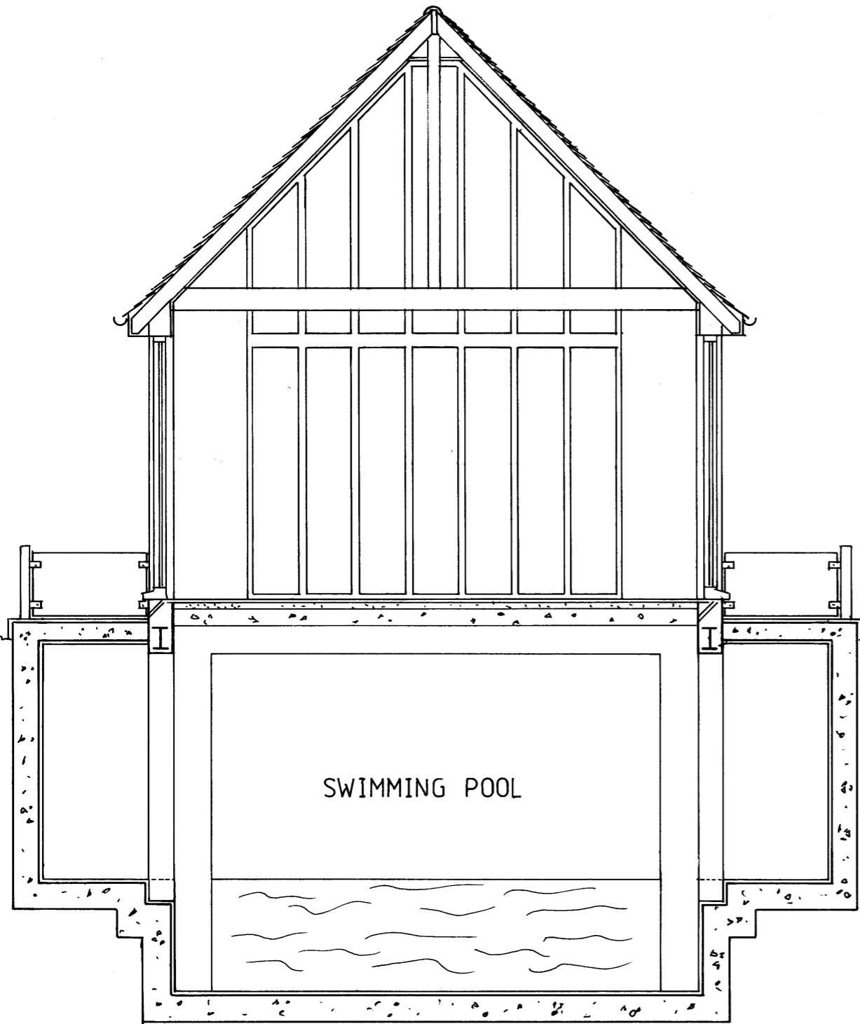
SECTION Y-Y
