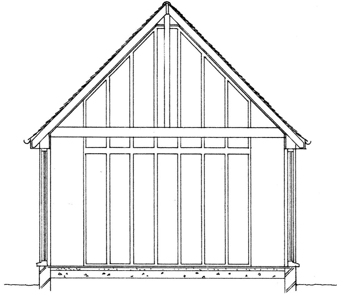
SECTION B-B
