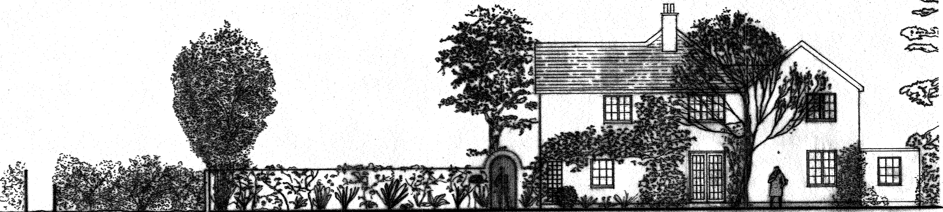
EASTERN ELEVATION
