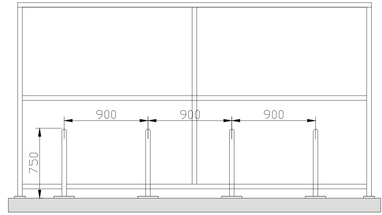
Proposed Cycle Store Elevation Scale 1:25 @A1
