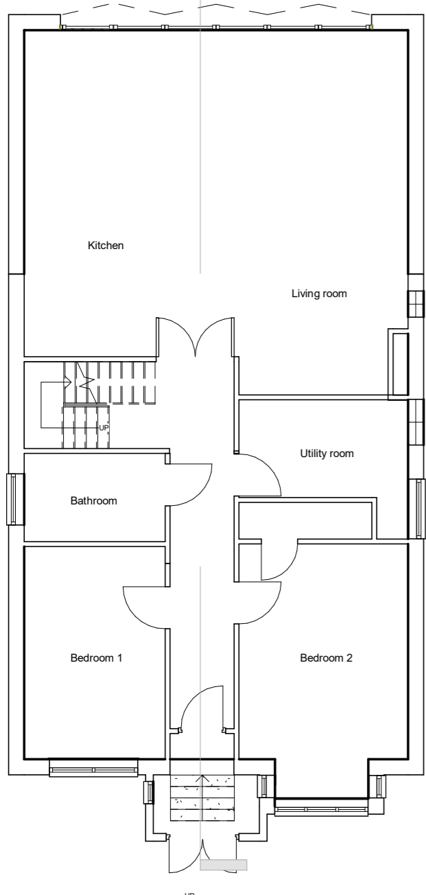
01. GF Pre-Existing 1 : 100
