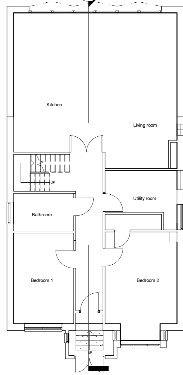
01. GF Proposed 1 : 100
