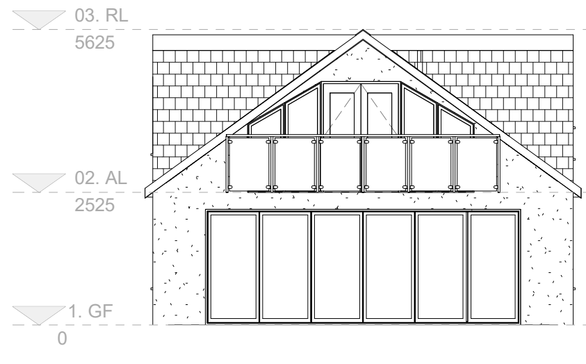
2. Rear Elevation Pre-existing 1 : 100
