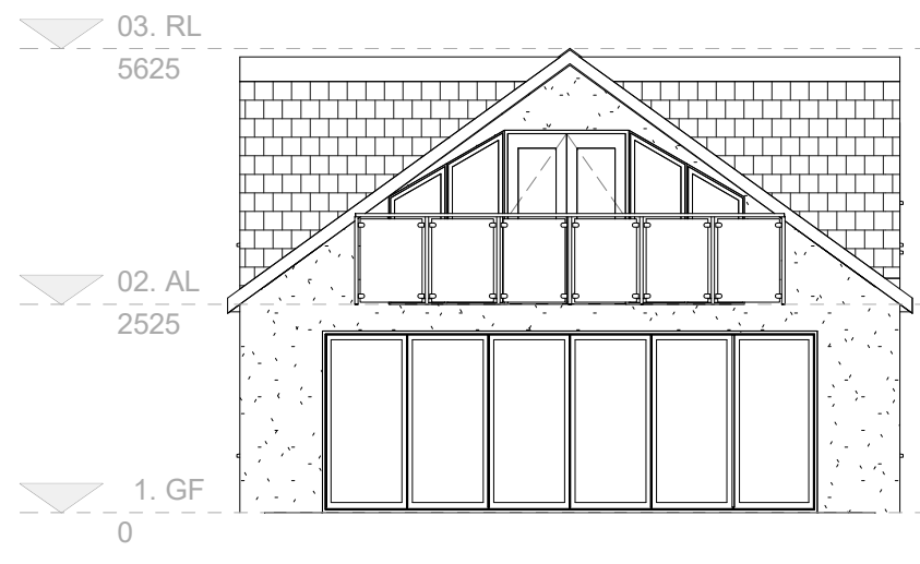
2. Rear Elevation Existing 1 : 100
