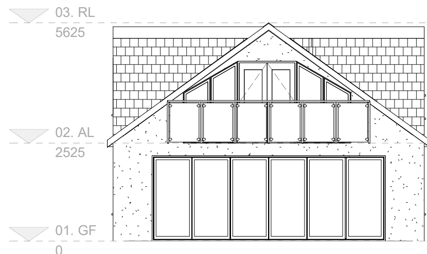
02. Rear Elevation Existing 1 : 100
