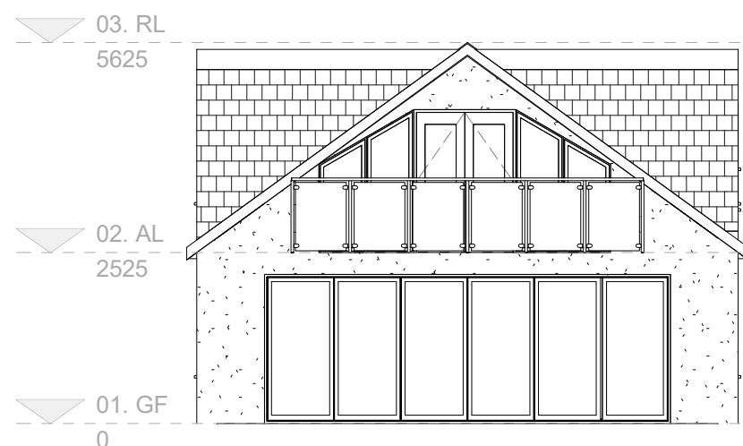
02. Rear Elevation Proposed 1 : 100
