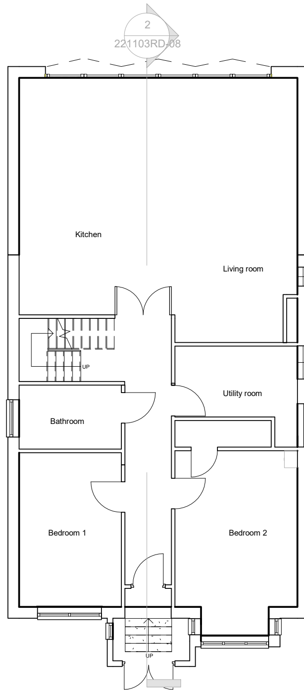
01. GF Proposed 1 : 100
