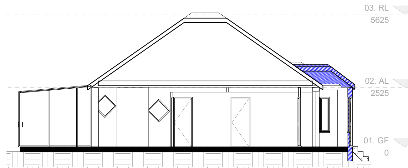
Section Proposed 1 : 100
