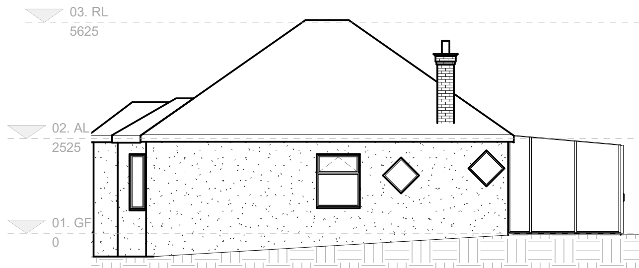
03. Right Elevation Proposed 1 : 100
