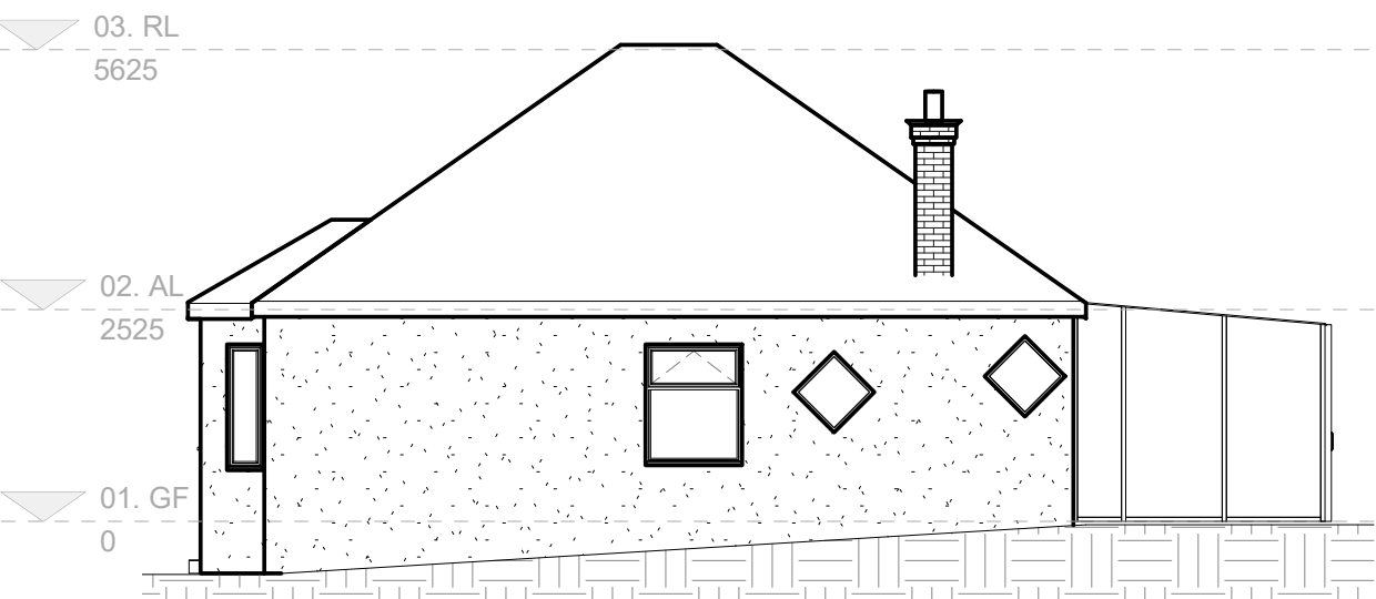
03. Right Elevation Existing 1 : 100
