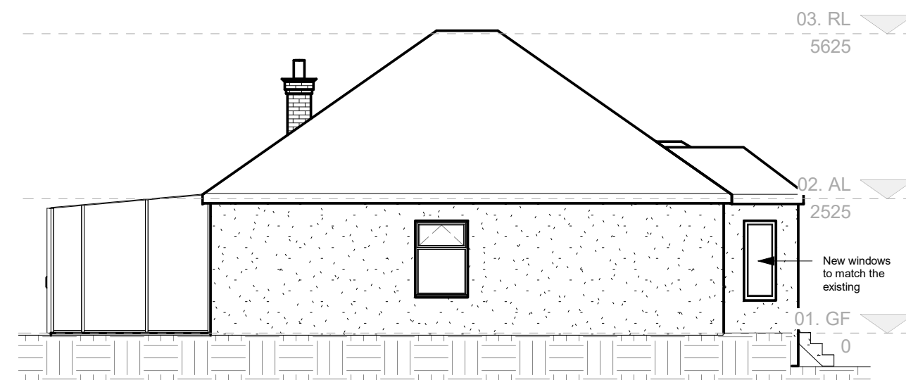
04. Left Elevation Proposed 1 : 100
