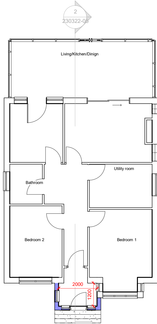
01. GF Proposed 1 : 100
