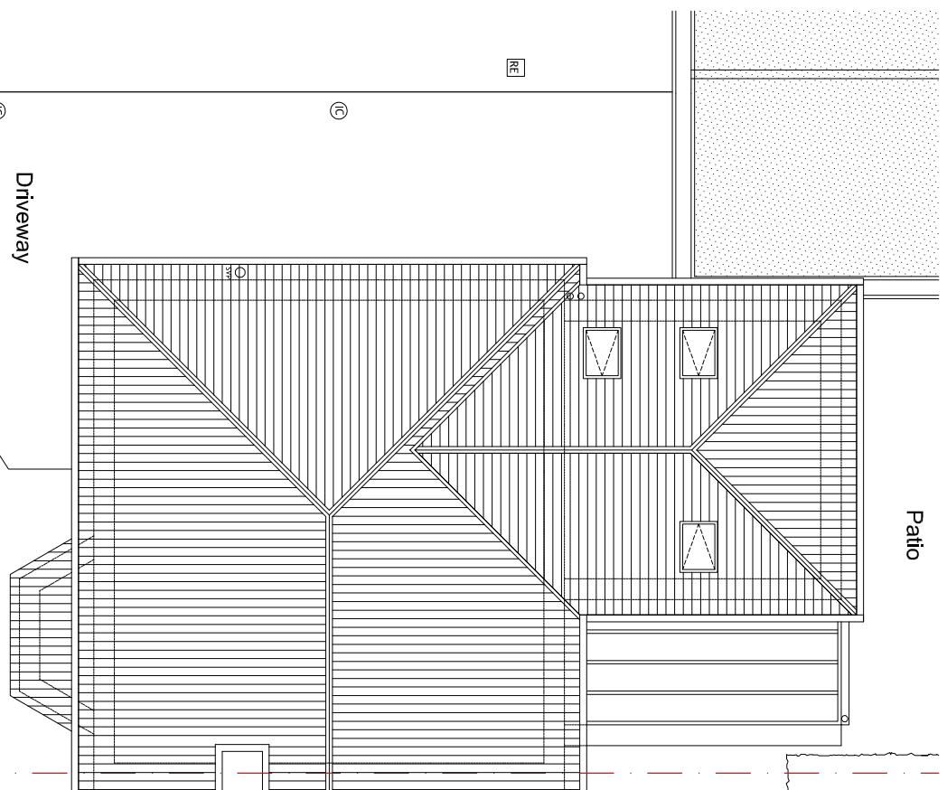
PROPOSED SITE/ROOF PLAN 1:200
