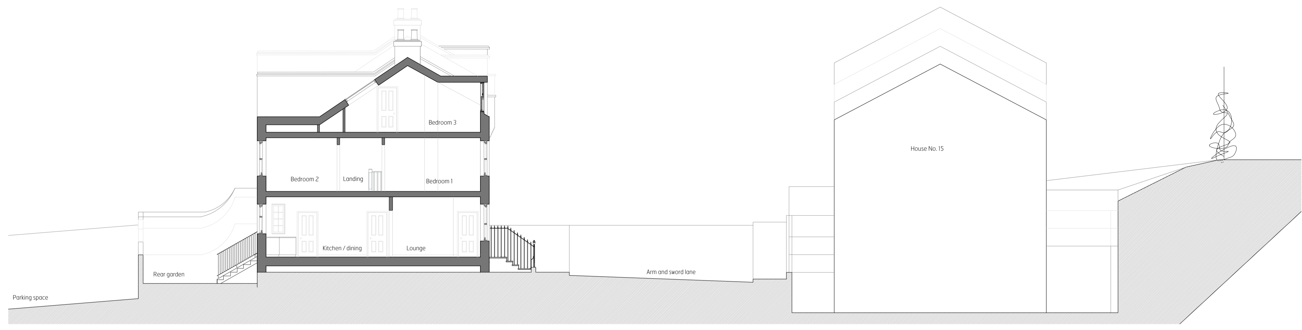
Proposed Section AA 1:100@A1 / 1:200@A3
